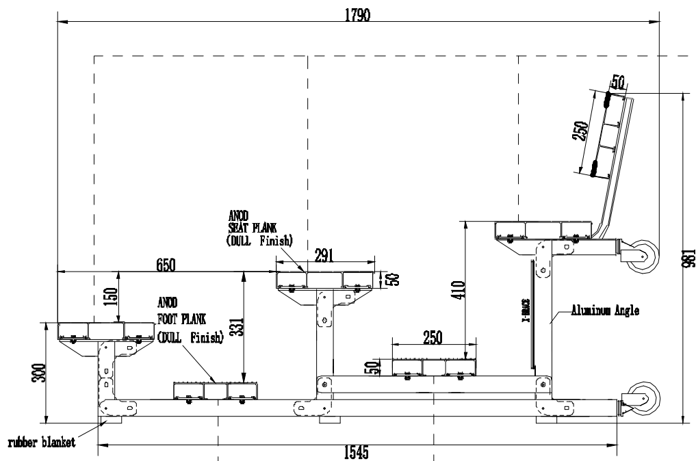
Side view AA
